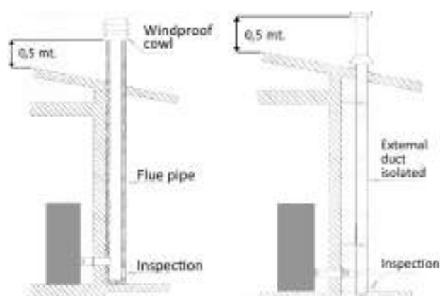
Fig. 2: connection to the flue pipe.
